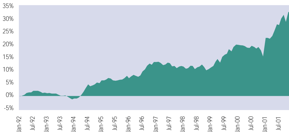
Figure 3: Rebalanced versus non-rebalanced index, cumulative outperformance
