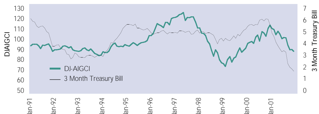
Figure 5: DJ-AIGCI versus 3 month treasury bill
